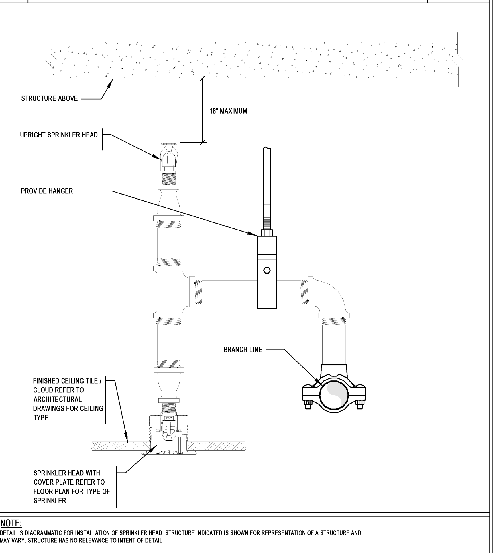
10 CONCEALED SPRINKLER WITH UPRIGHT SPRINKLER SCALE: NOT TO SCALE
