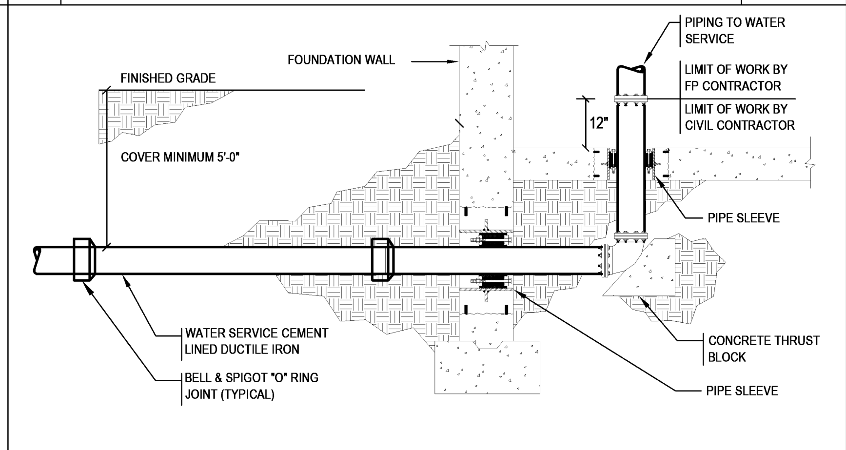
7 FIRE SERVICE THROUGH FLOOR SCALE: NOT TO SCALE
