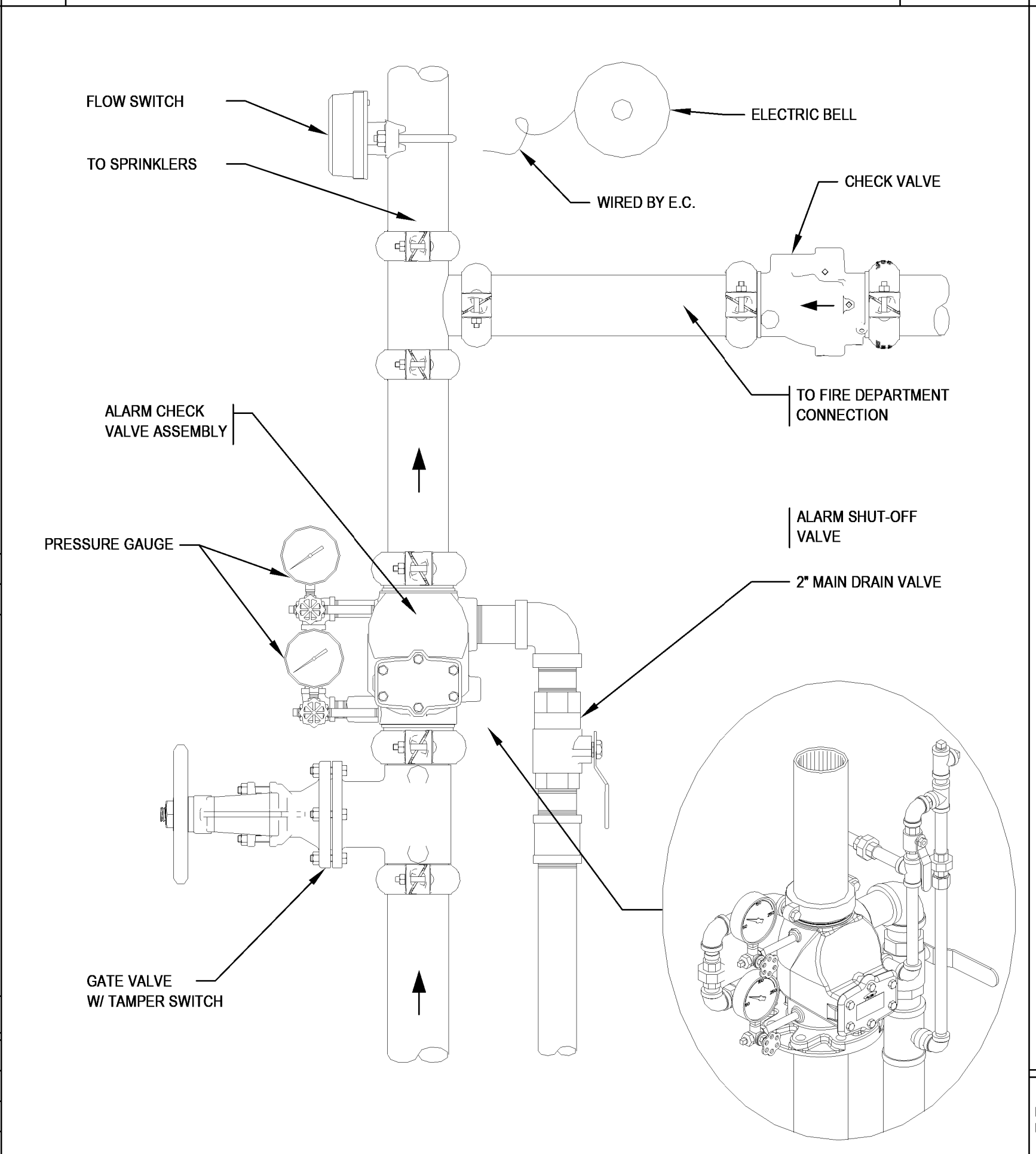
9 WET SPRINKLER ALARM VALVE SCALE: NOT TO SCALE
